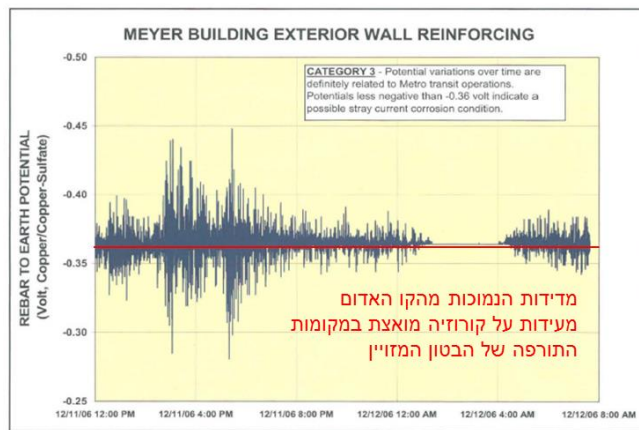
FIGURE 6 – Sample Stray Current Data, Significance Category 3
